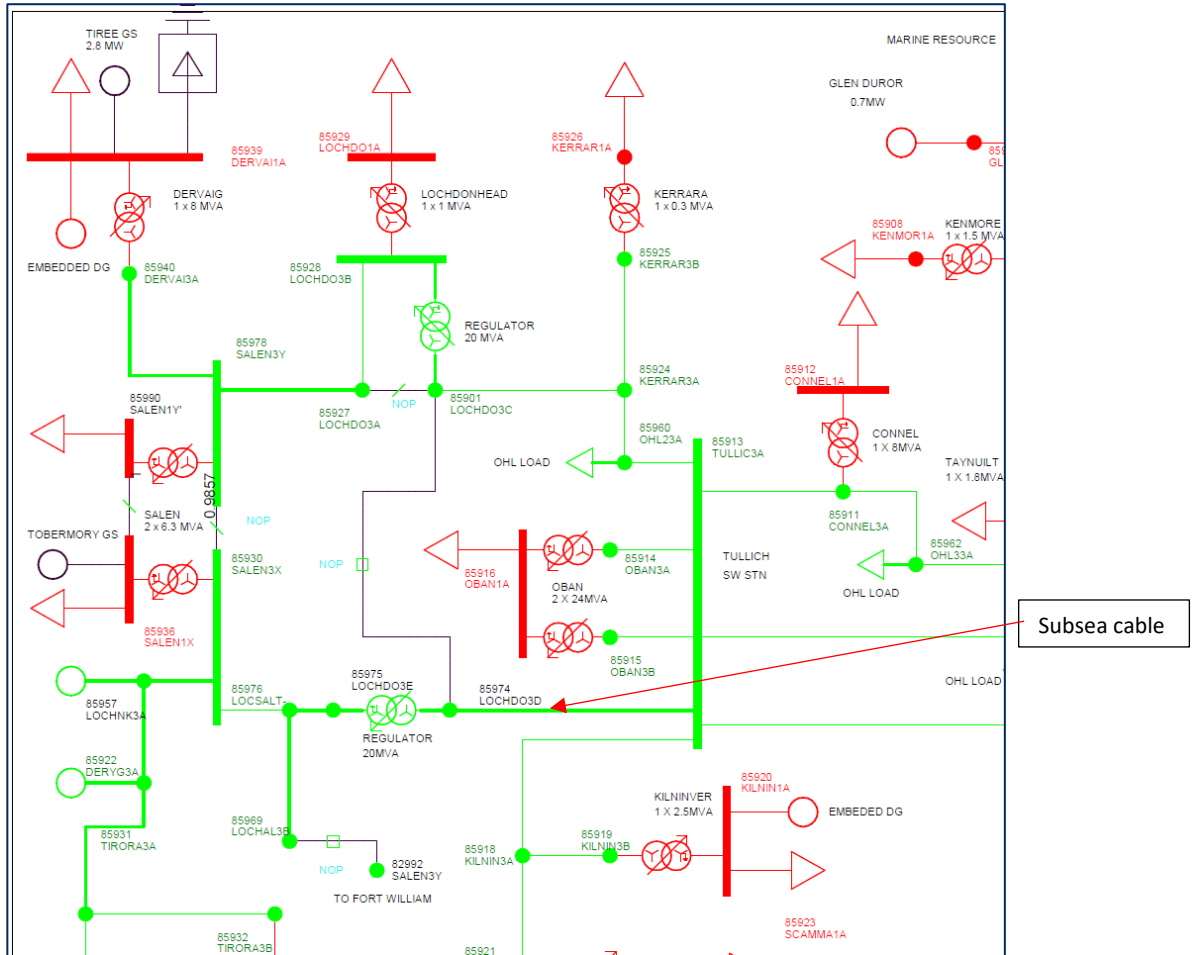
Figure 3: Mainland – Kerrera 2 Network Arrangement SLD.
