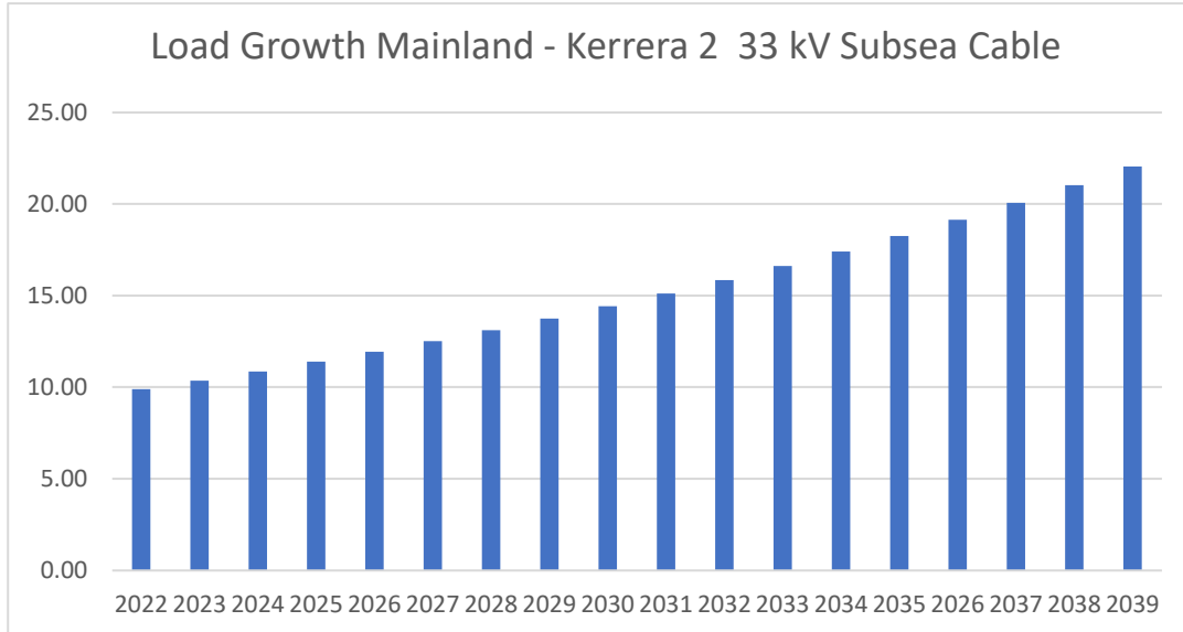
Figure 2- Load Forecast Mainland - Kerrera - 33 kV Feeder
